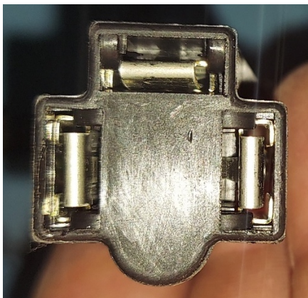
Low-beam headlight connector.
